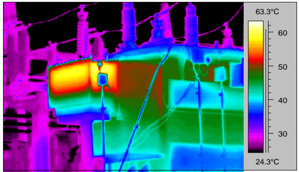
INTERNAL PROBLEM ON LOAD TAP CHANGER
