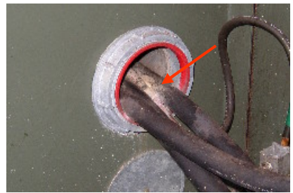
CORONA "DUST" ON 13KV CONDUCTOR
