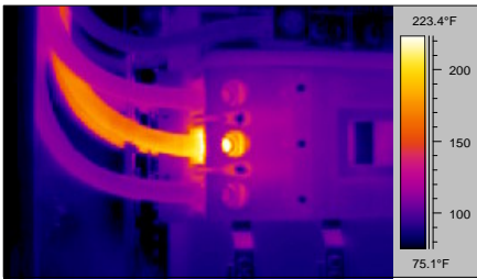
LOOSE CONDUCTOR CONNECTION
