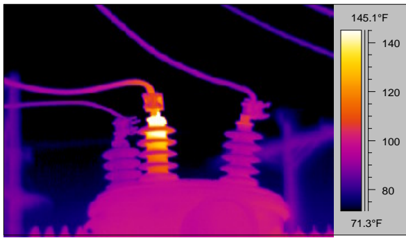
INTERNAL PROBLEM ON VOLTAGE REGULATOR BUSHING
