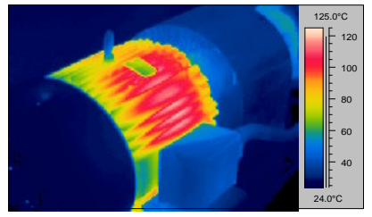
SINGLE-PHASED 100HP MOTOR
